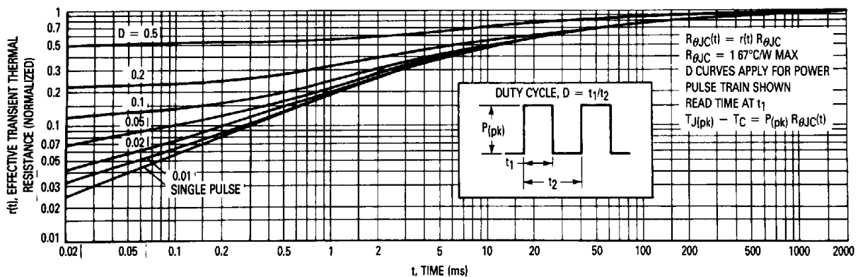
Figure 10. Thermal Response
