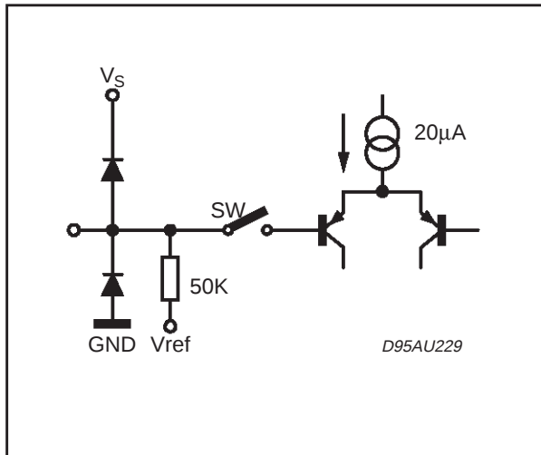
Figure 15. Pin: L-OUT, R-OUT, MONITOR-L, MONITOR-R, LTR OUTPUT, BASSO-L, BASSO-R, AUXOUT_L, AUXOUT_R
