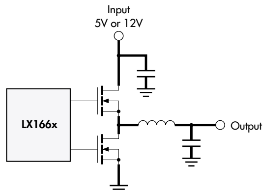
FIGURE 13 — Power Traces
