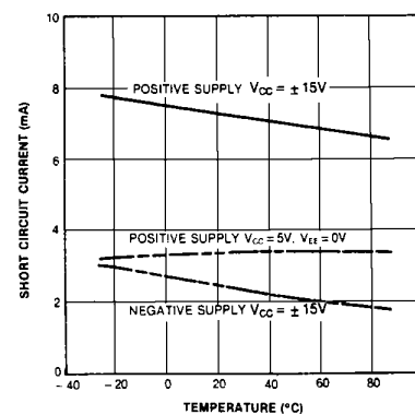
Figure 10. Supply Current
