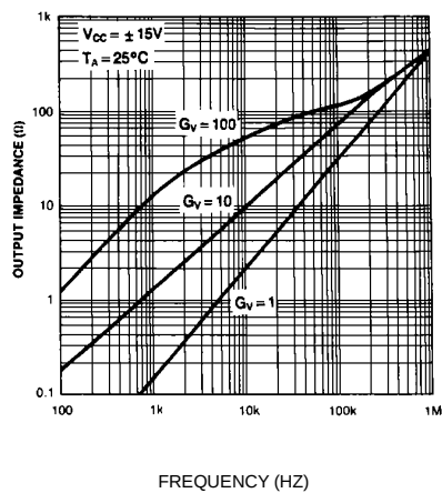
Fig. 5 OUTPUT IMPEDANCE
