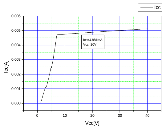
Figure 1. V_{CC} - I_{CC}
