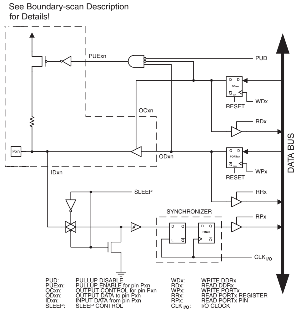
Figure 128. General Port Pin Schematic Diagram
