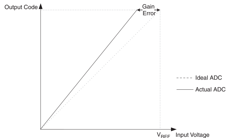
Figure 118. Gain Error
