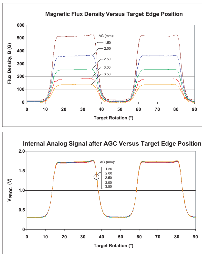
Figure 7. Effect of AGC. The upper panel shows the magnetic gradient detected at the Hall element, with no amplification. The lower panel displays the corresponding internal processed signal, V_{PROC} . This normalized electrical signal allows optimal performance by the rest of the circuits that reference this signal.
