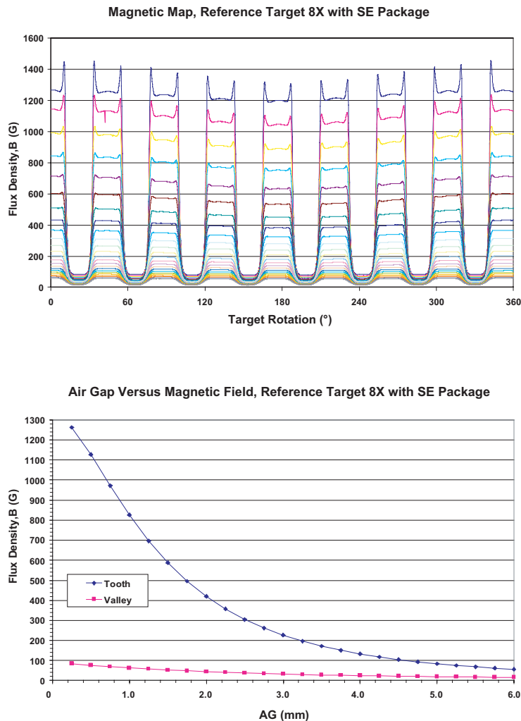
Figure 10. Magnetic Data for the 8X Reference Target and SE package.
