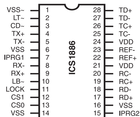
28-Pin SOLC
