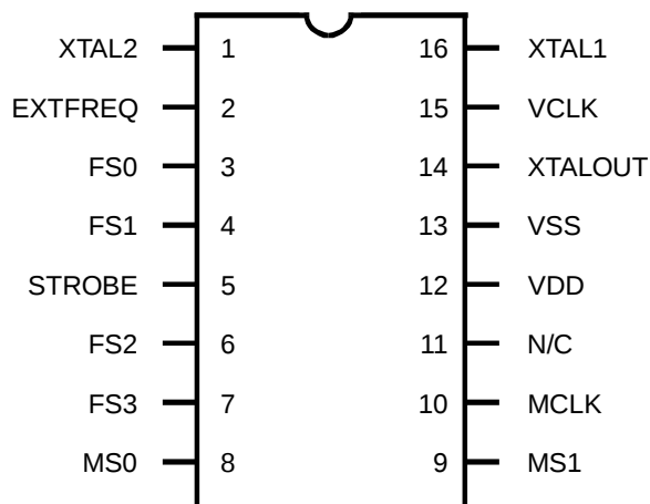
16-Pin DIP or SOIC
