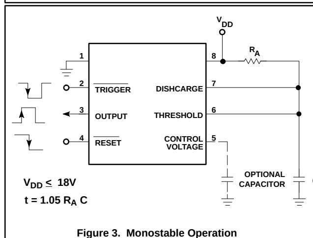
Figure 3. Monostable Operation
