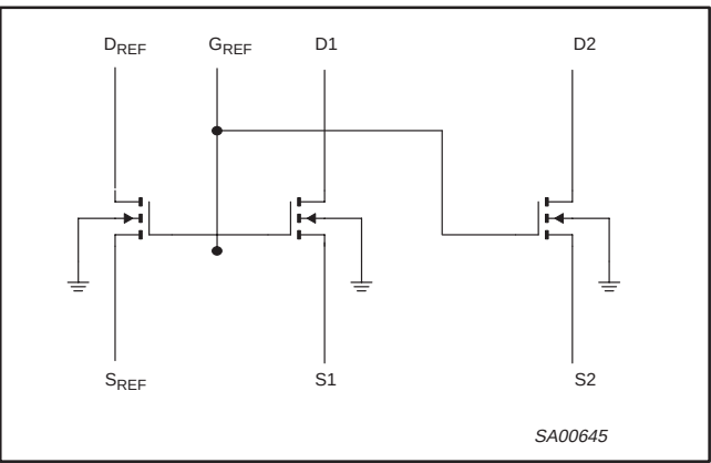
Figure 3. Clamp schematic
