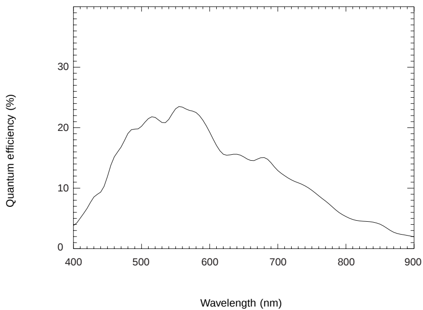
Figure 5 - Quantum efficiency versus wavelength
