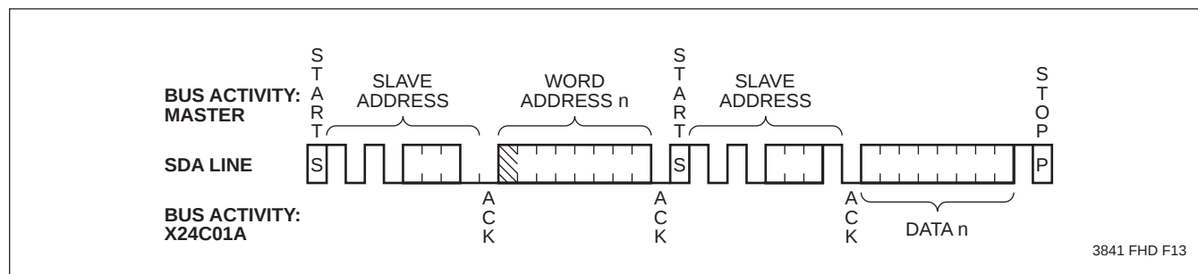
Figure 8. Random Read
