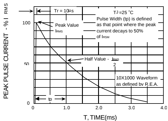
FIG.5 - PULSE WAVEFORM
