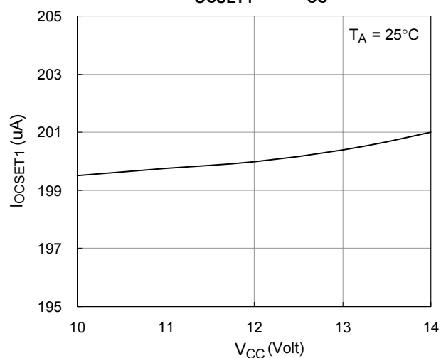
I_{OCSET1} vs. V_{CC}
