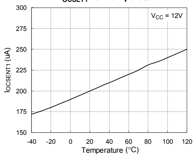
I_{OCSET1} vs. Temperature
