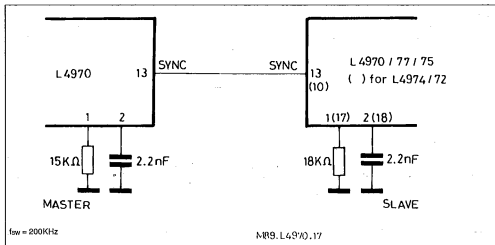
Figure 34 : L4970's Sync. Example.
