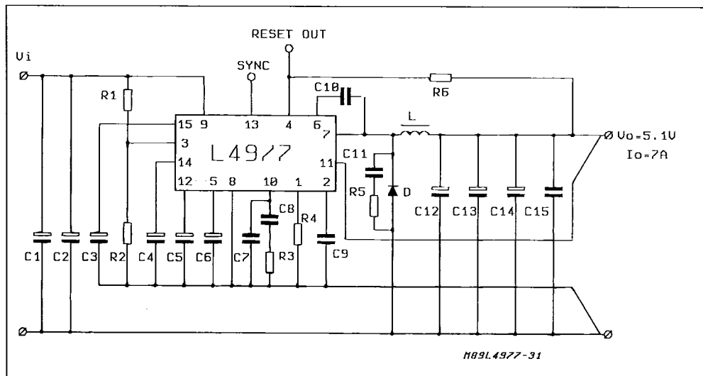
Figure 32 : 7A - 5.1V Application Circuit.
