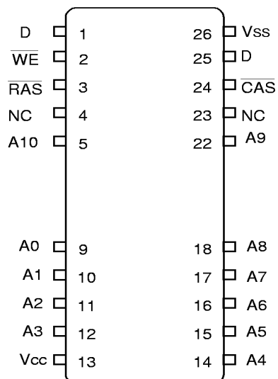
20/26 Pin Plastic TSOP- II (300mil)
