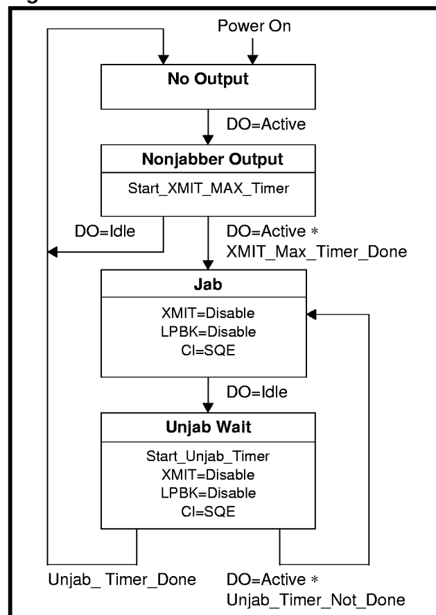
Figure 3: Jabber Control Function
