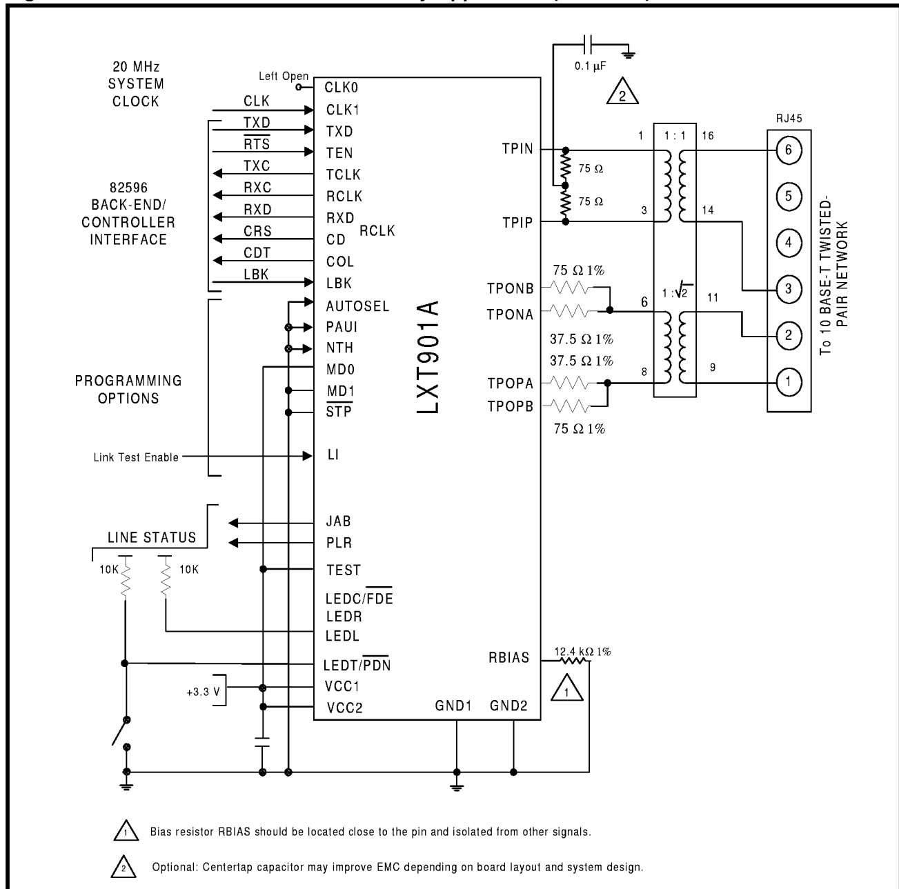
Figure 15: 150 \Omega Shielded Twisted-Pair Only Application (LXT901A)
