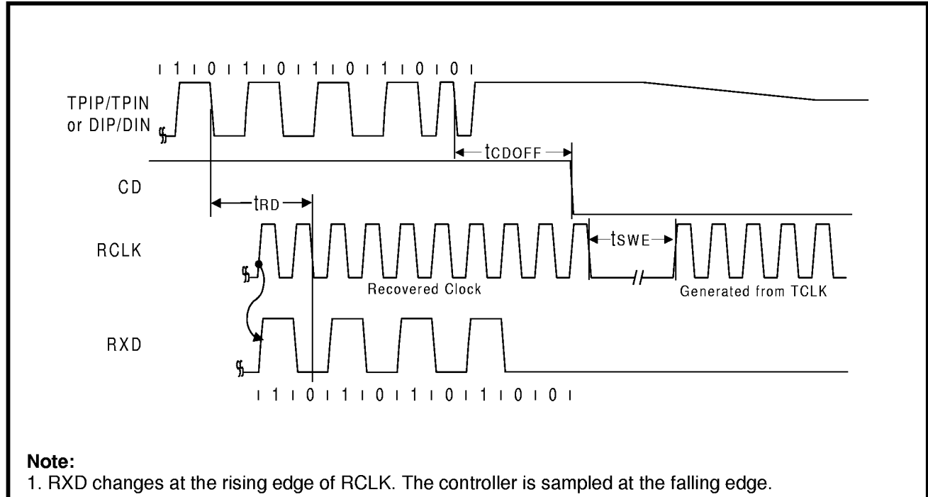
Figure 31: Mode 3 RCLK/End-of-Frame Timing (LXT907A)
