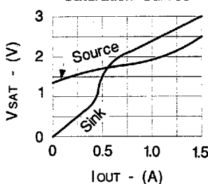
Saturation Curves
