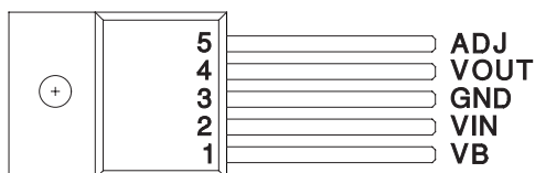
5-Pin TO-220 (Top View) T Package
