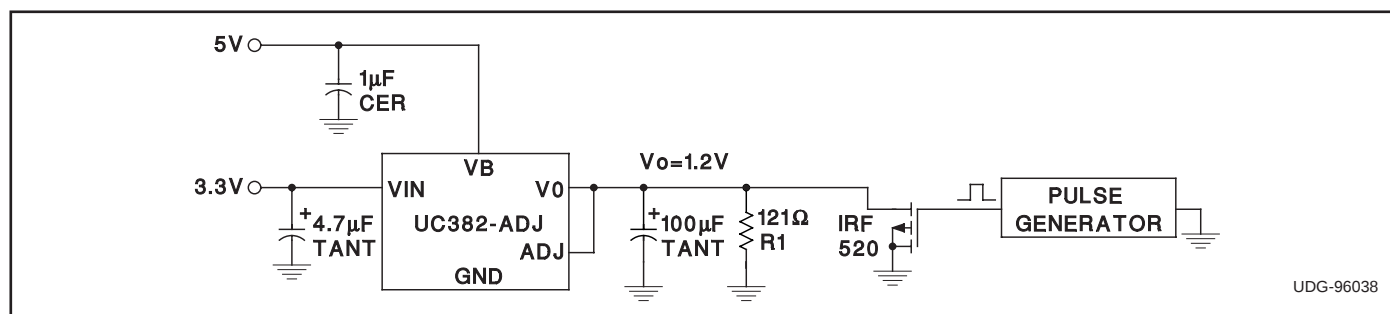
Figure 6. Transient test circuit.
