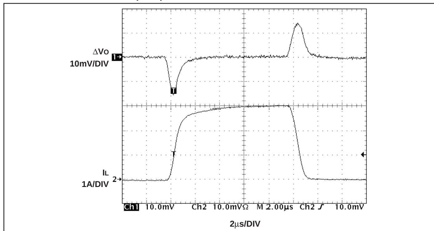
Figure 7. 10mA to 3A/μs load transient response.
