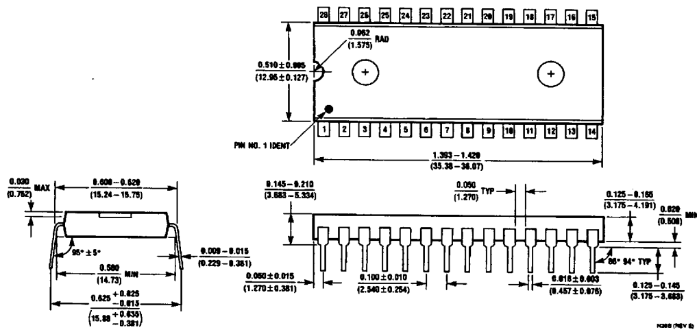
Molded Dual-In-Line Package (N) Order Number DP8570AN NS Package Number N28B
