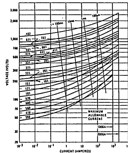
Fig. 5 - Voltage Vs. Current Characteristics, Z15L Series
