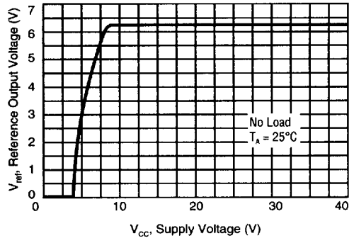
REFERENCE OUTPUT VOLTAGE versus SUPPLY VOLTAGE
