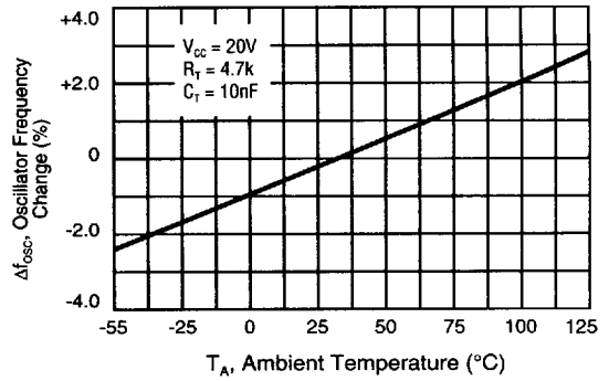
OSCILLATOR FREQUENCY CHANGE versus TEMPERATURE
