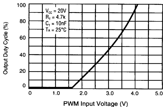
OUTPUT DUTY CYCLE versus PWM INPUT VOLTAGE
