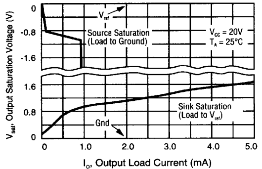
ERROR AMP OUTPUT SATURATION VOLTAGE versus LOAD CURRENT
