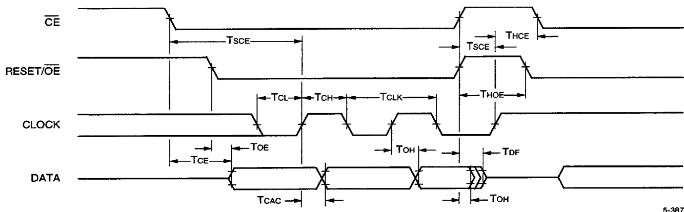
Figure 4. Read Characteristics
