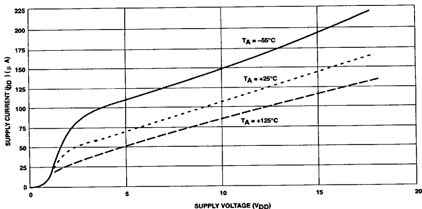
Supply Current vs Supply Voltage
