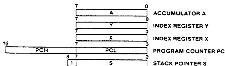
Figure 3. Microprocessor Programming Model
