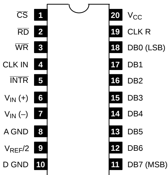
Pin Connection Diagram
