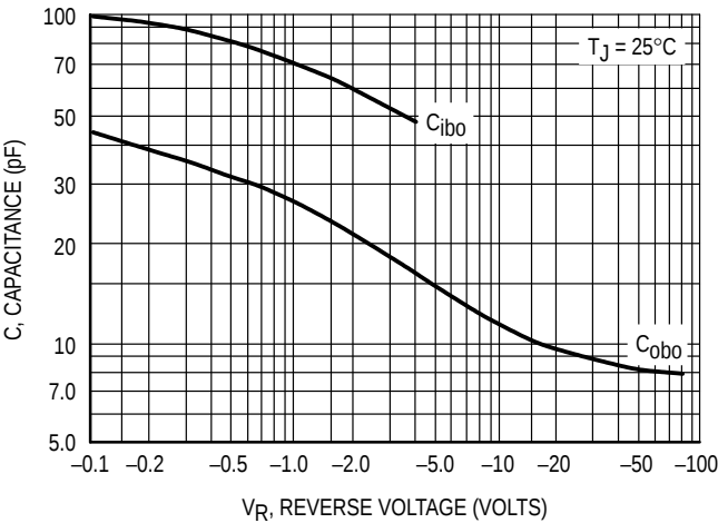
Figure 5. MPSA55/56 Capacitance
