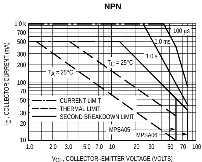
Figure 8. MPSA05/06 Active-Region Safe Operating Area
