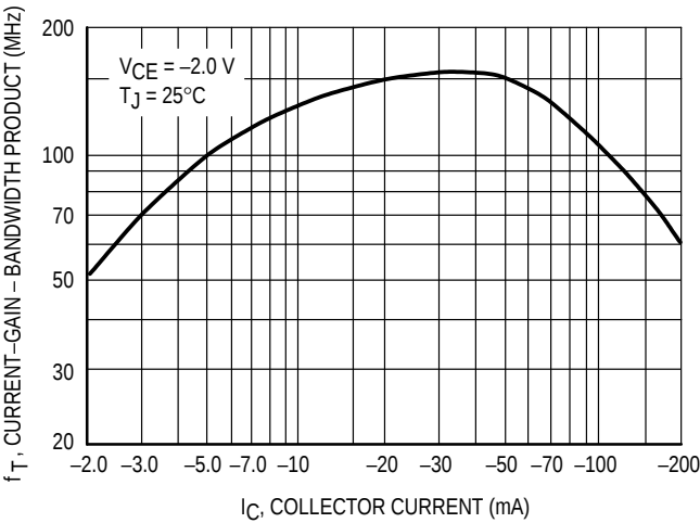
Figure 3. MPSA55/56 Current-Gain — Bandwidth Product
