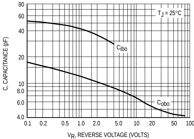
Figure 4. MPSA05/06 Capacitance
