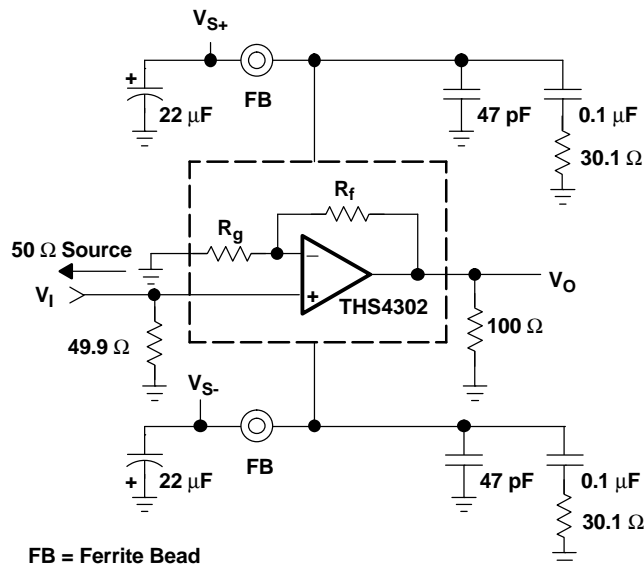
APPLICATION CIRCUIT
