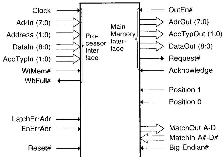
Figure 1 Logic Symbol
