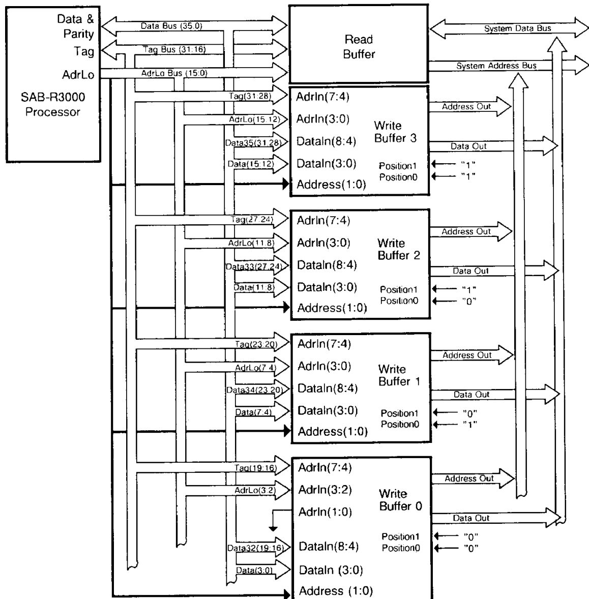
Figure 5 Write Buffer Data and Address Line Connections
