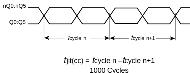
CYCLE-TO-CYCLE JITTER
