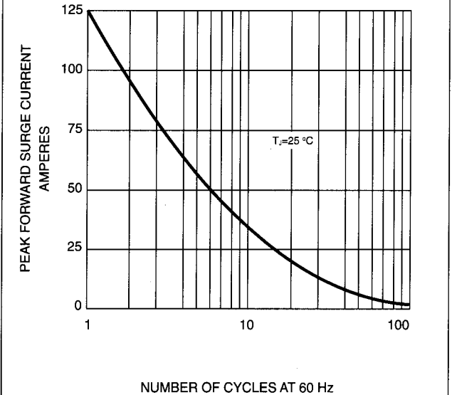
FIG. 3-MAXIMUM FORWARD SURGE CURRENT
