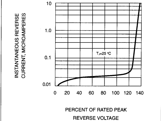
FIG. 2-TYPICAL REVERSE CHARACTERISTICS
