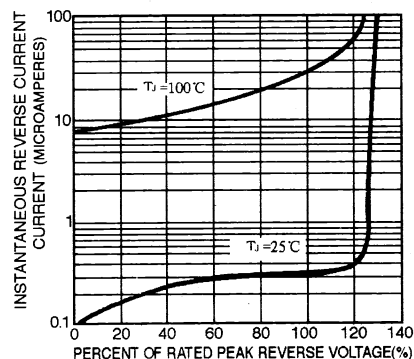
FIG.4 - TYPICAL REVERSE CHARACTERISTICS PER ELEMENT
