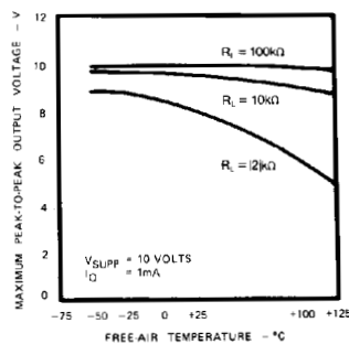
MAXIMUM PEAK-TO-PEAK OUTPUT VOLTAGE AS A FUNCTION OF FREE-AIR TEMPERATURE
