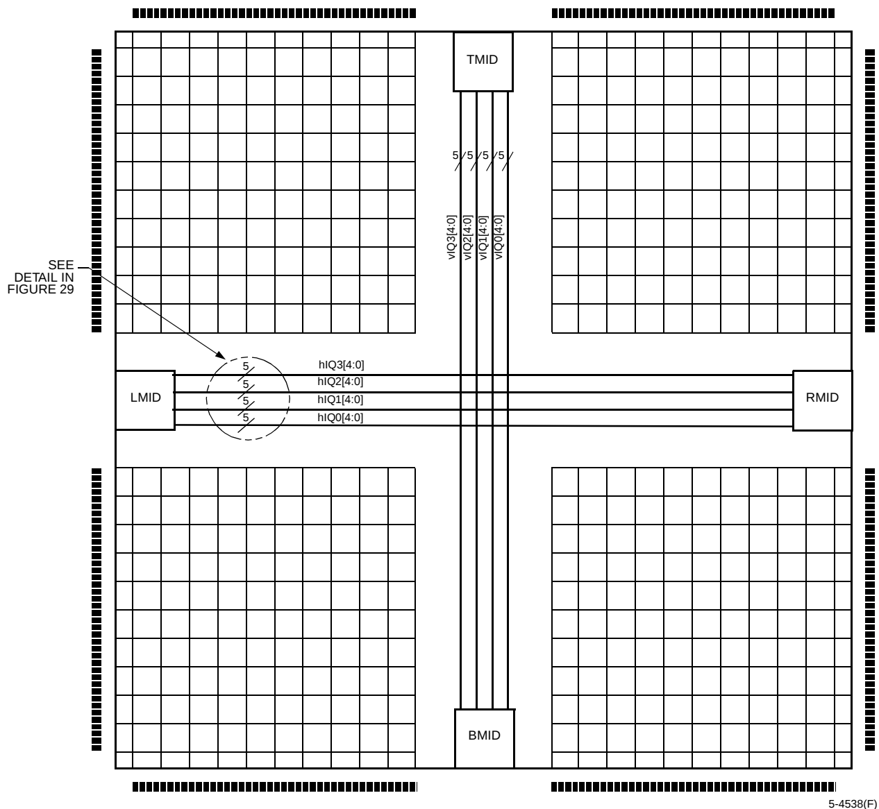
Figure 28. Interquad Routing
