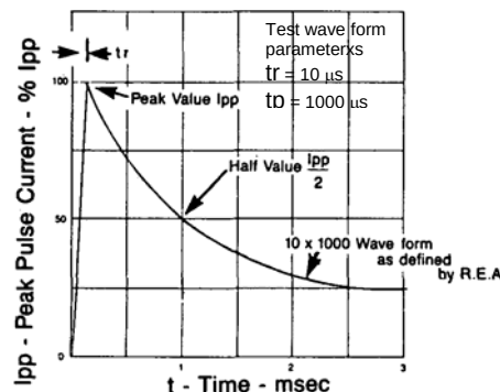
FIGURE 2 PULSE WAVEFORM
