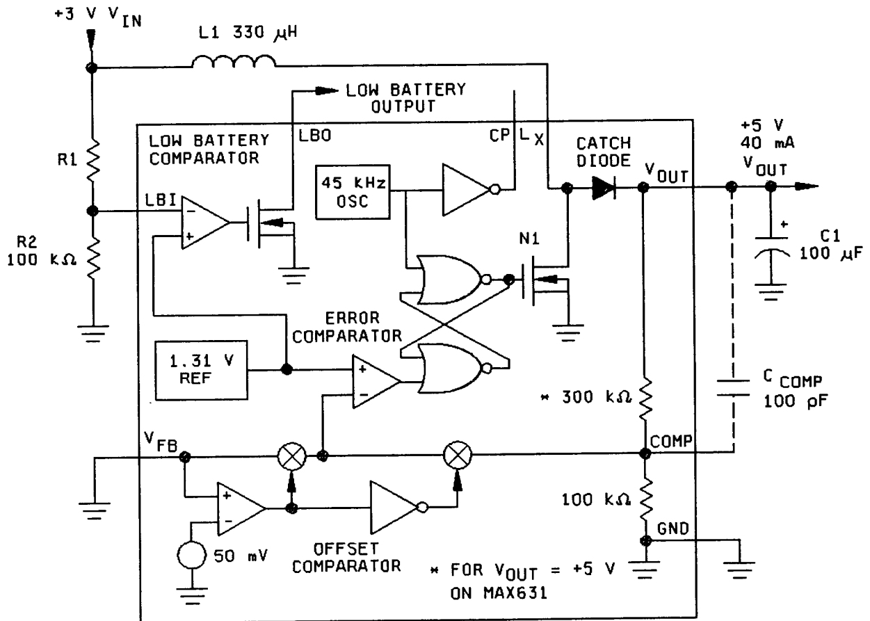
FIGURE 2. Block diagram.
