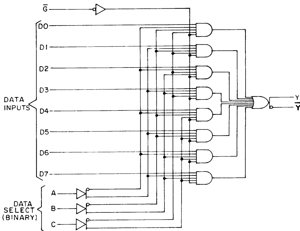
FIGURE 3. Logic diagram.
