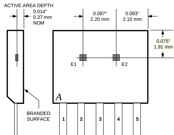
Figure 5 SENSOR LOCATIONS ( \pm 0.005" [0.13 mm] die placement)
