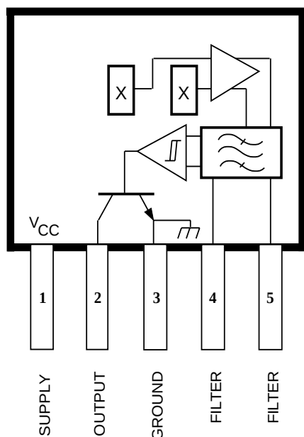
Dwg. PH-011
