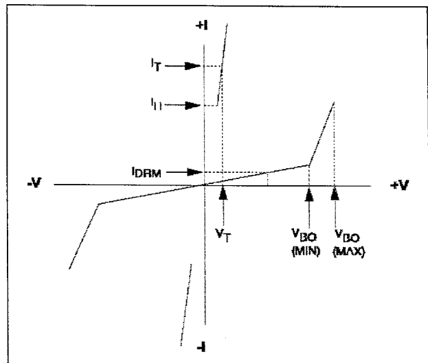
V-I Characteristics
