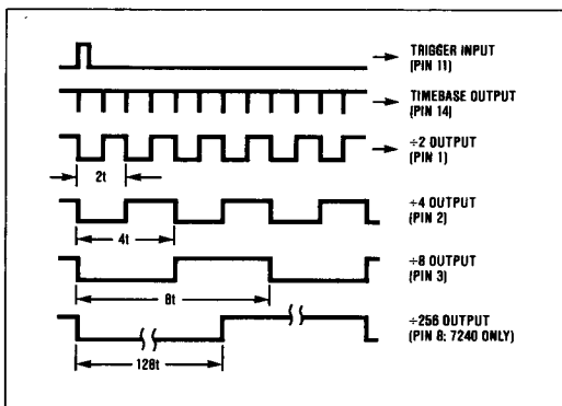
Figure 1. Timing Diagram for ICM7240/50/60.
