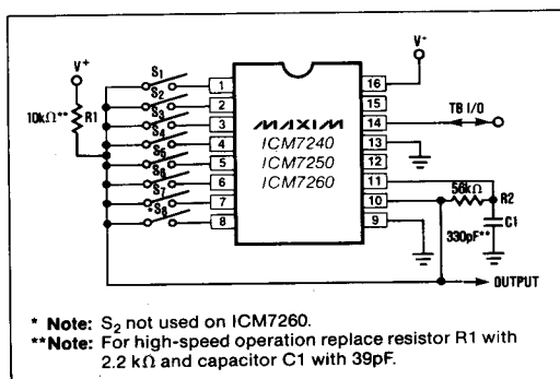
Figure 3. Programming the Counter Section of the ICM7240/50/60
