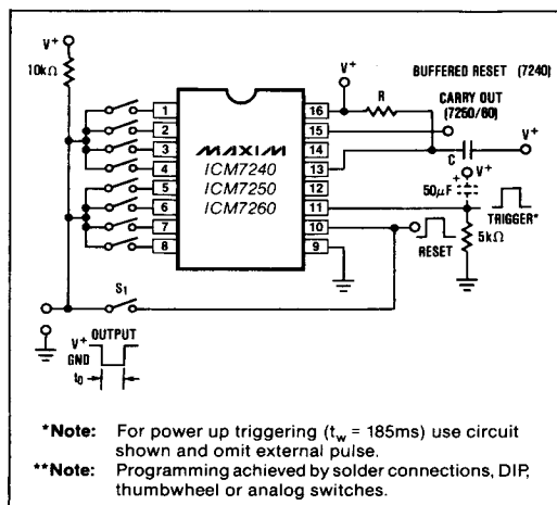
Figure 2. Generalized Circuit for Timing Applications (Switch S_1 open for astable operation, closed for monostable operation)
