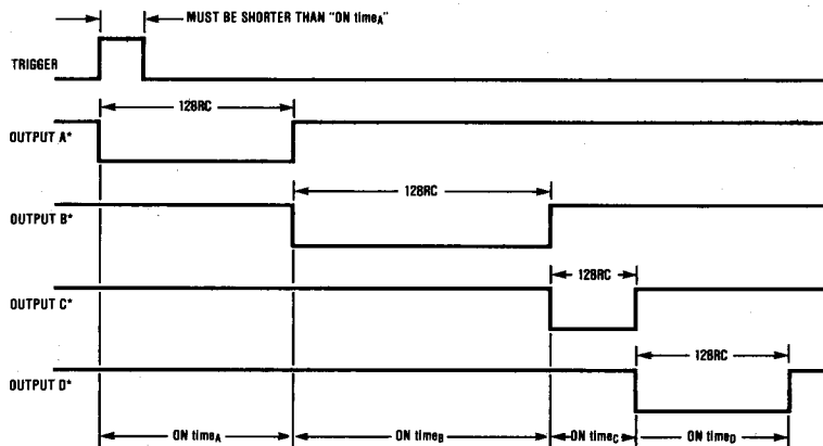
Figure 5. Timing Diagram for Sequence Timer of Figure 4.
