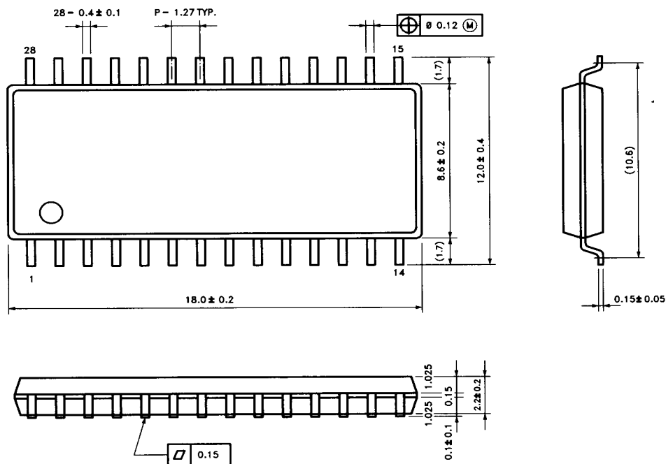
Figure 3. 28-Lead Small Out-Line Package (PG)
