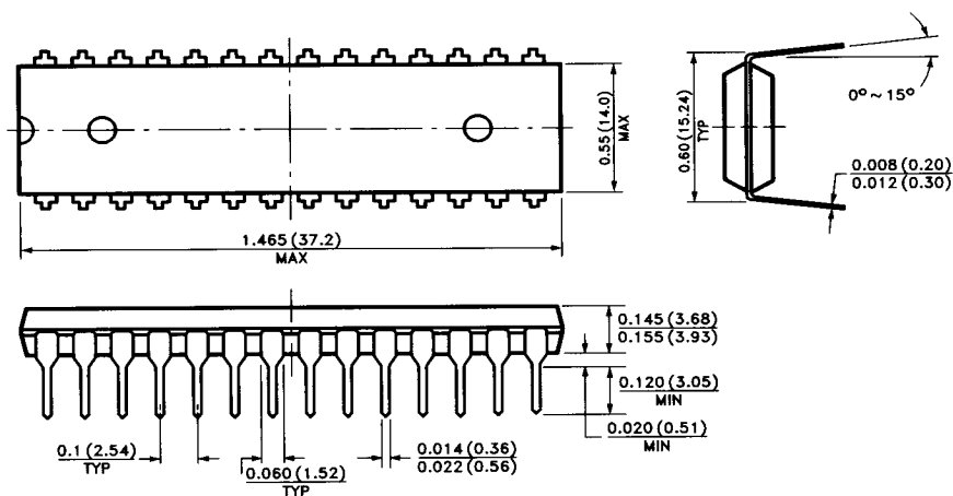
Figure 2. 28-Lead Plastic Dual In-Line Package (P)
