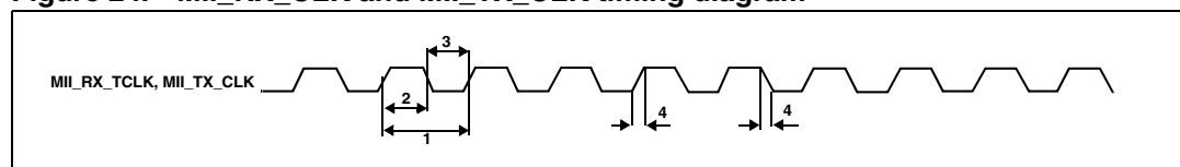
Figure 24. MII_RX_CLK and MII_TX_CLK timing diagram
