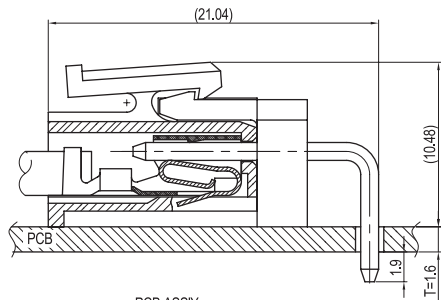
PCB ASSY
