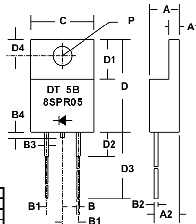
FULLY INSULATED PACKAGE
