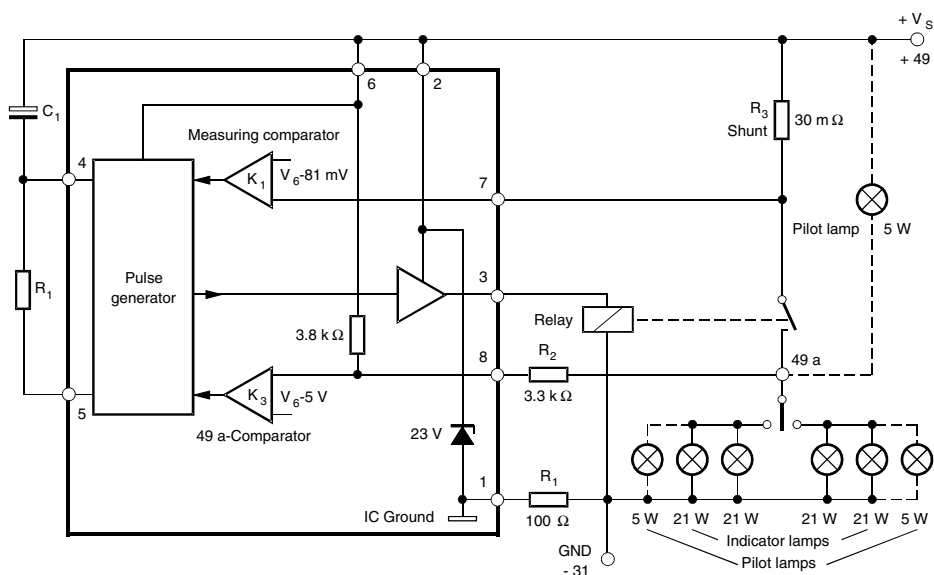
Figure 1-1. Block Diagram
