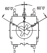
RTE03* 3 POSITION
