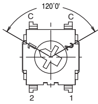
RTE02* 2 POSITION
