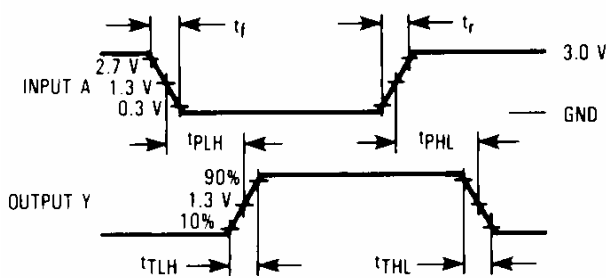
Figure 1. Switching Waveforms
