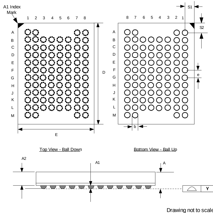
Figure 4. 256-Mbit, 88-ball (80-active ball) SCSP Drawing and Dimensions (8x11x1.0 mm)
