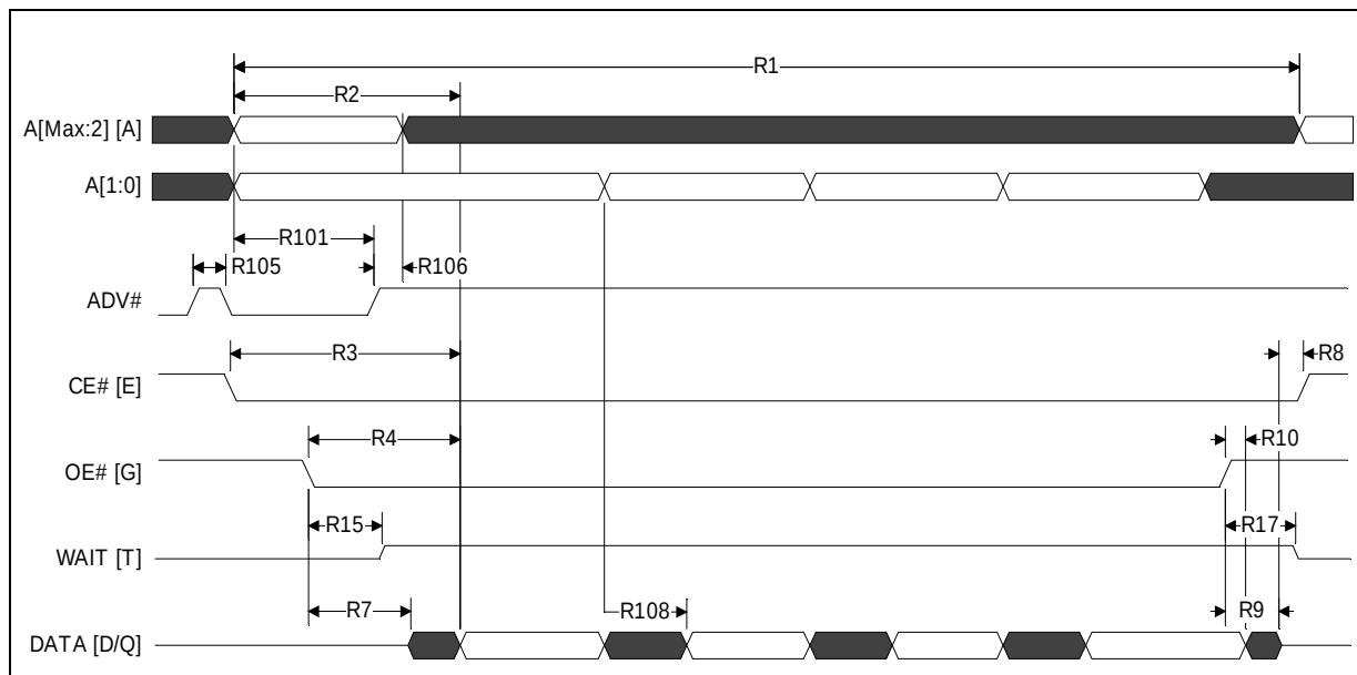
Figure 13. Asynchronous Page-Mode Read Timing
